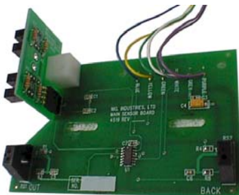
T-15094521 Sensor Board
