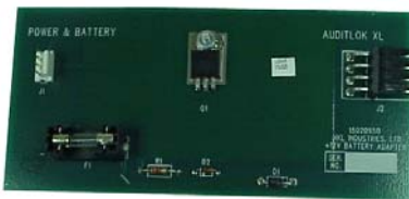
T-15020950 Power Supply Step-Down Board
