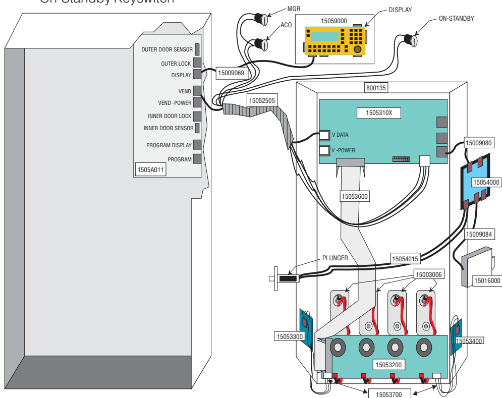
D8X Electronics Assembly Diagram
